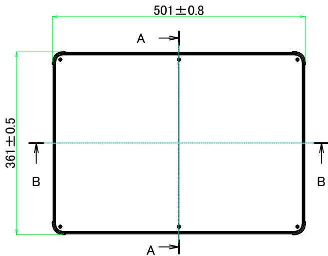
E view
