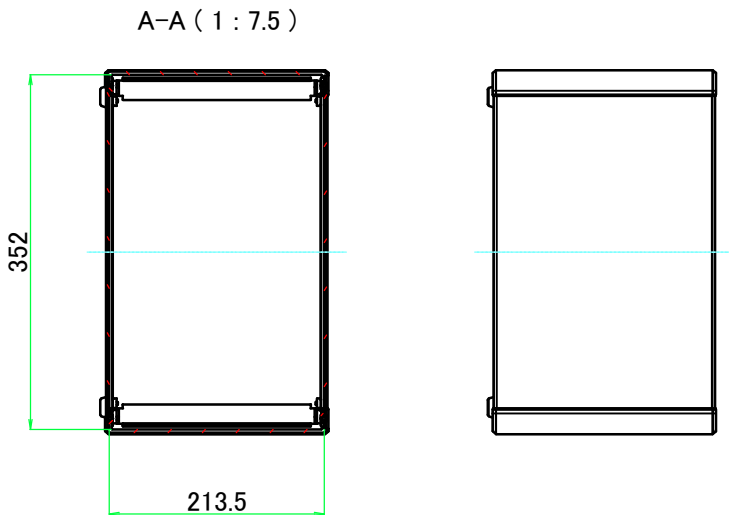
D view
